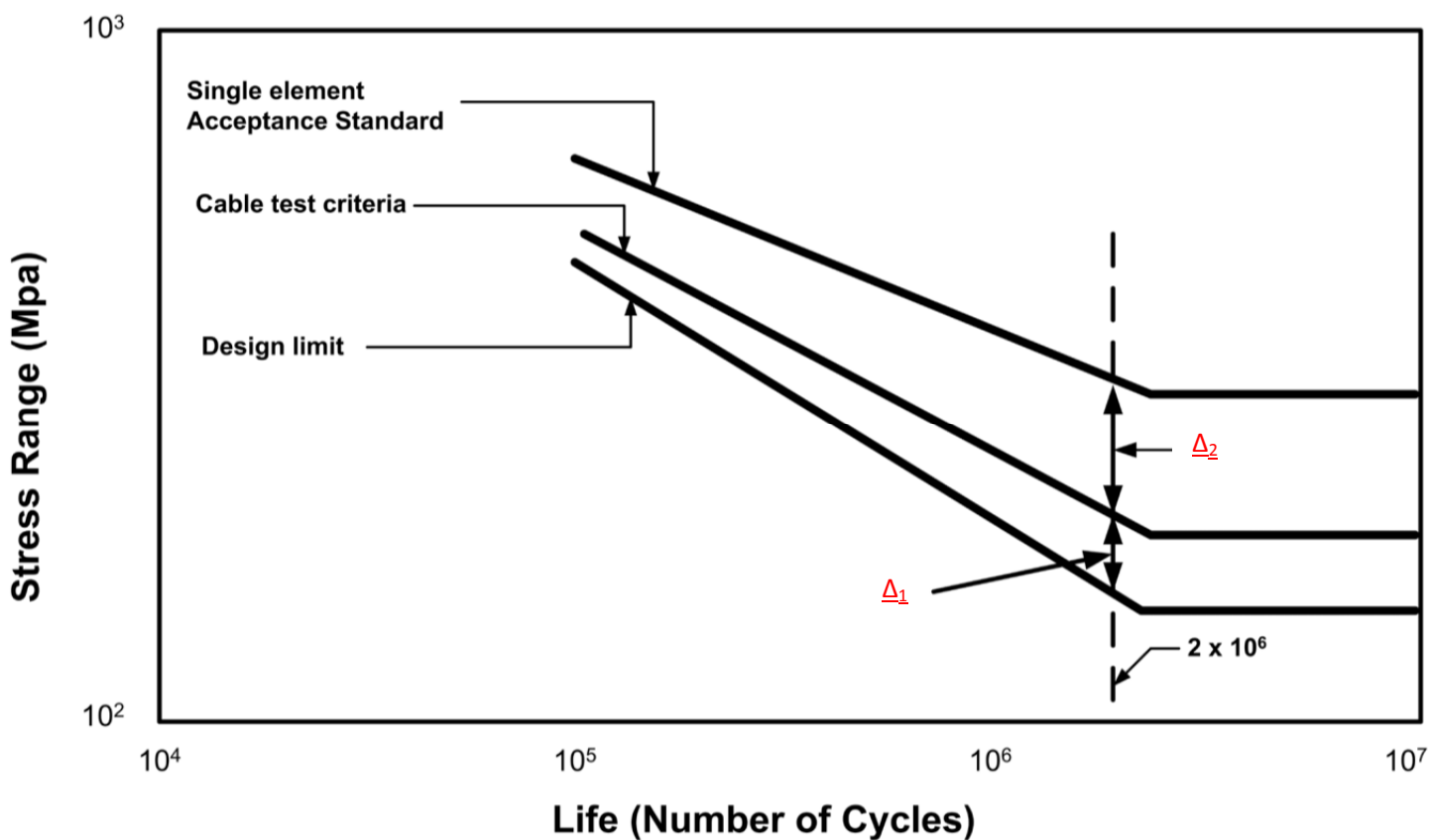
Fig. C3.1 – Fatigue safety philosophy. (Note: \Delta_1 is quality assurance [17 MPa coupled bar, 69 MPa strand and uncoupled bar, 103 MPa wire] and \Delta_2 is length effect, anchorage riser, safety [35 MPa].)
