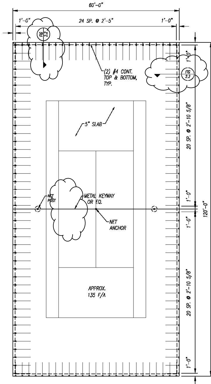
Page 62, Section 16.0 – EXAMPLE PLANS, Fig. 16 (a) – Layout of post-tensioning tendons in single court.
