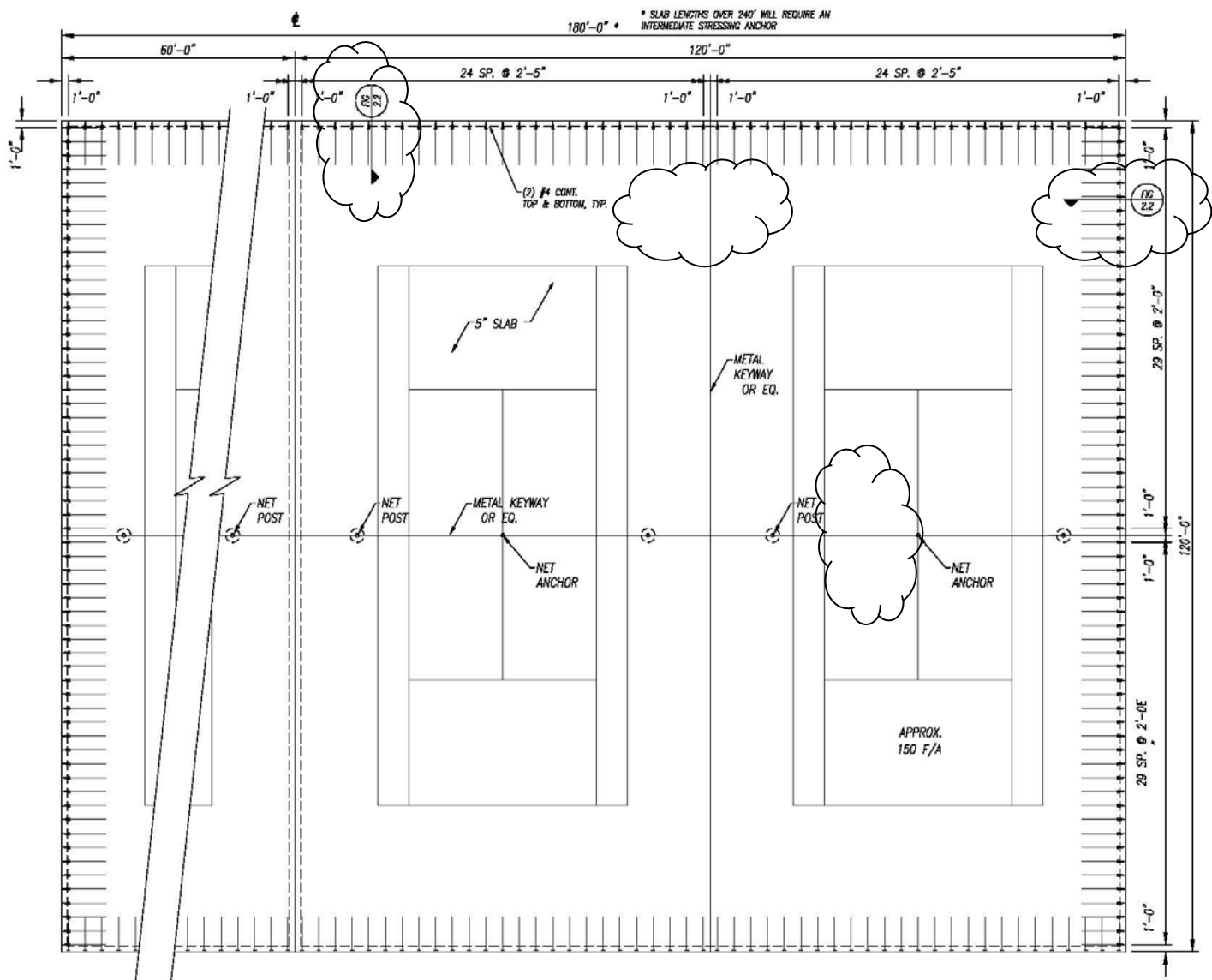
Page 65, Section 16.0 – EXAMPLE PLANS, Fig. 16 (d) – Layout of post-tensioning tendons in a quadruple or larger court.
